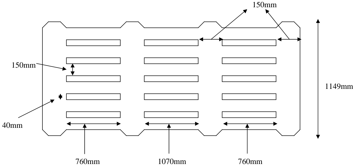
Figure 1 Overhead View
