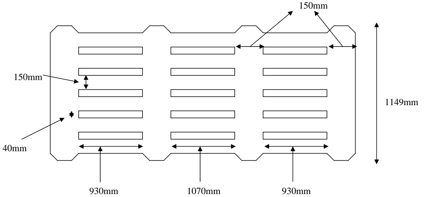
Figure 3 Overhead View
