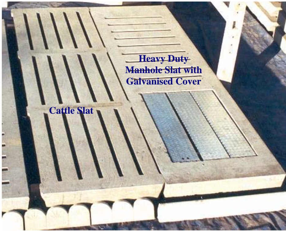
Figure 8 Slat photos
