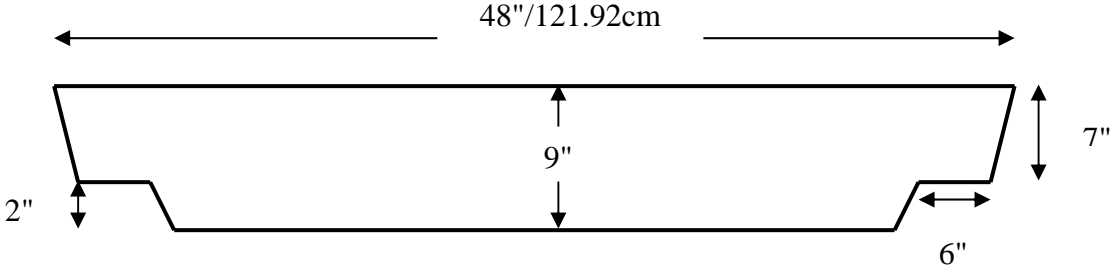
Figure 7 Side View of 9" stepped to 7" deep Manhole to suit Cattle Slats.
