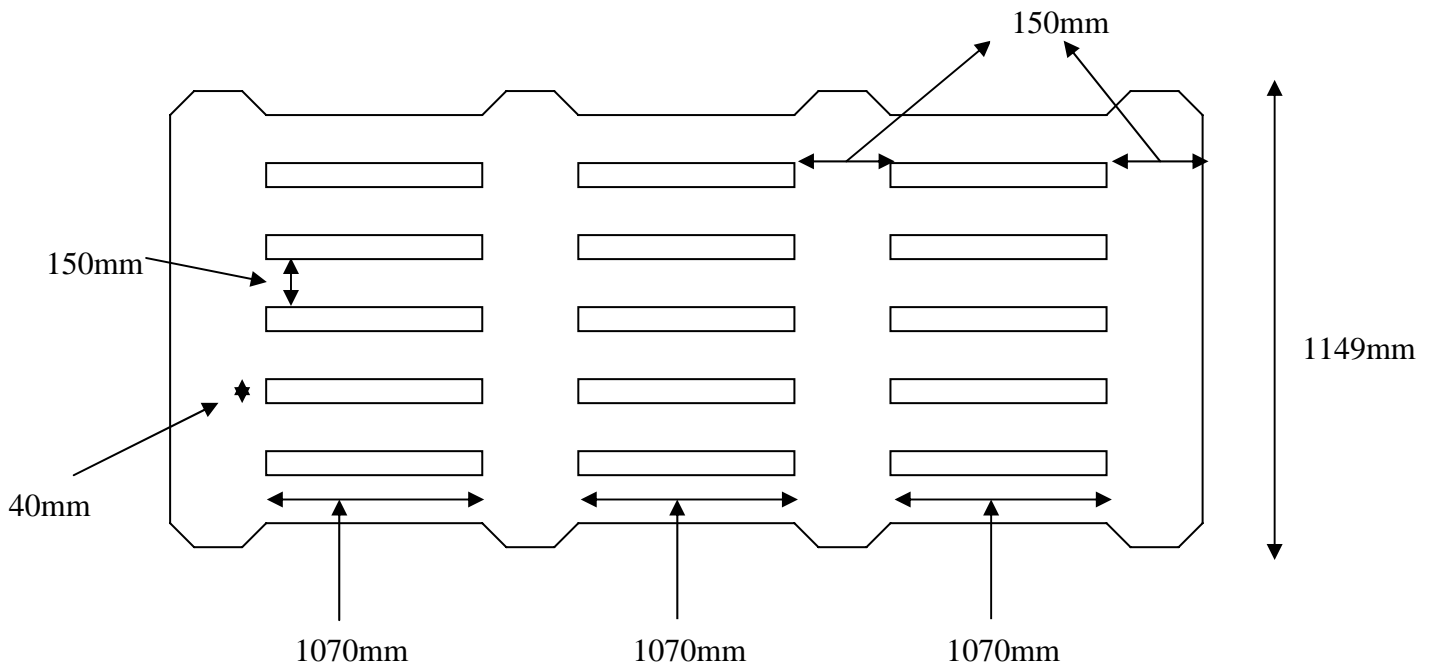
Figure 4 Overhead View
