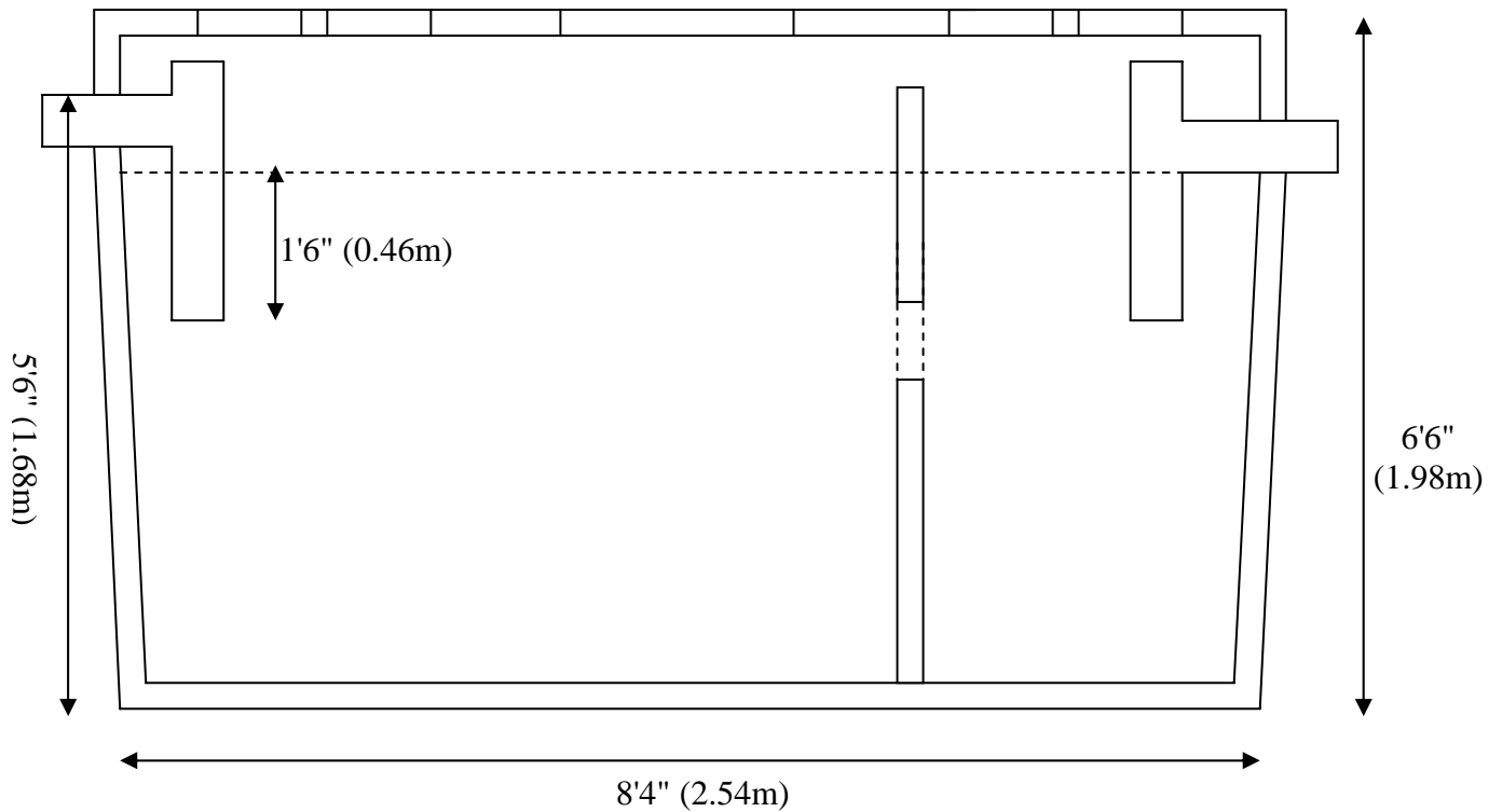
Sectional View
